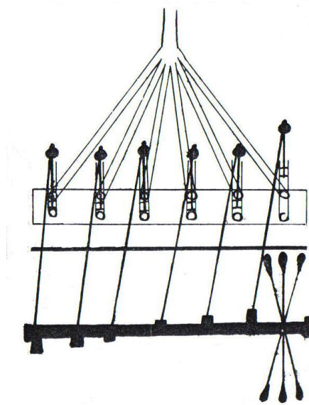
Figure 6: Drawing of the six-cylinder pump as it was depicted by Taqi al-Din in “The Sublime Methods of Spiritual Machines” (Chester Beatty Library in Dublin, Arabic MS 5232, p. 38) [19].
